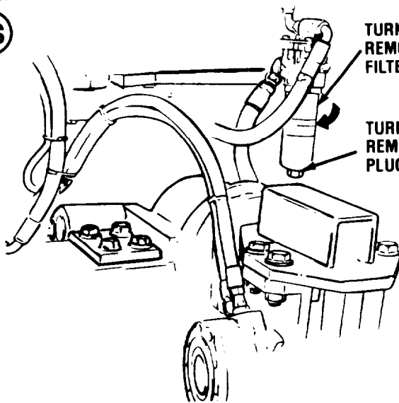
HYDRAULIC FLUID FILTER
