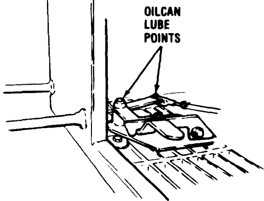
PUMP ENGAGEMENT LEVER
