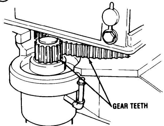
ROTATION GEAR BEARING AND PINION TEETH
