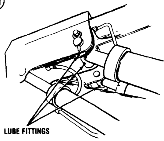
UPPER LIFT CYLINDER PIVOT
